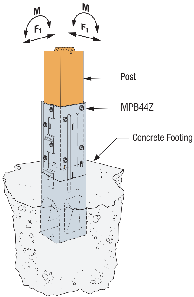
SIMPSON Strong-Tie® MPB44Z Installation
