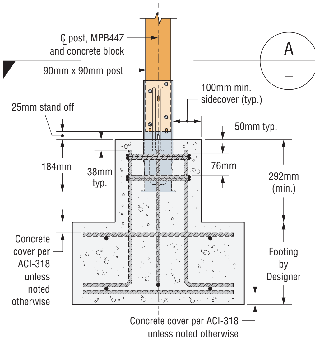
SIMPSON Strong-Tie® MPB44Z Reinforced Concrete Footing - Cross Section
