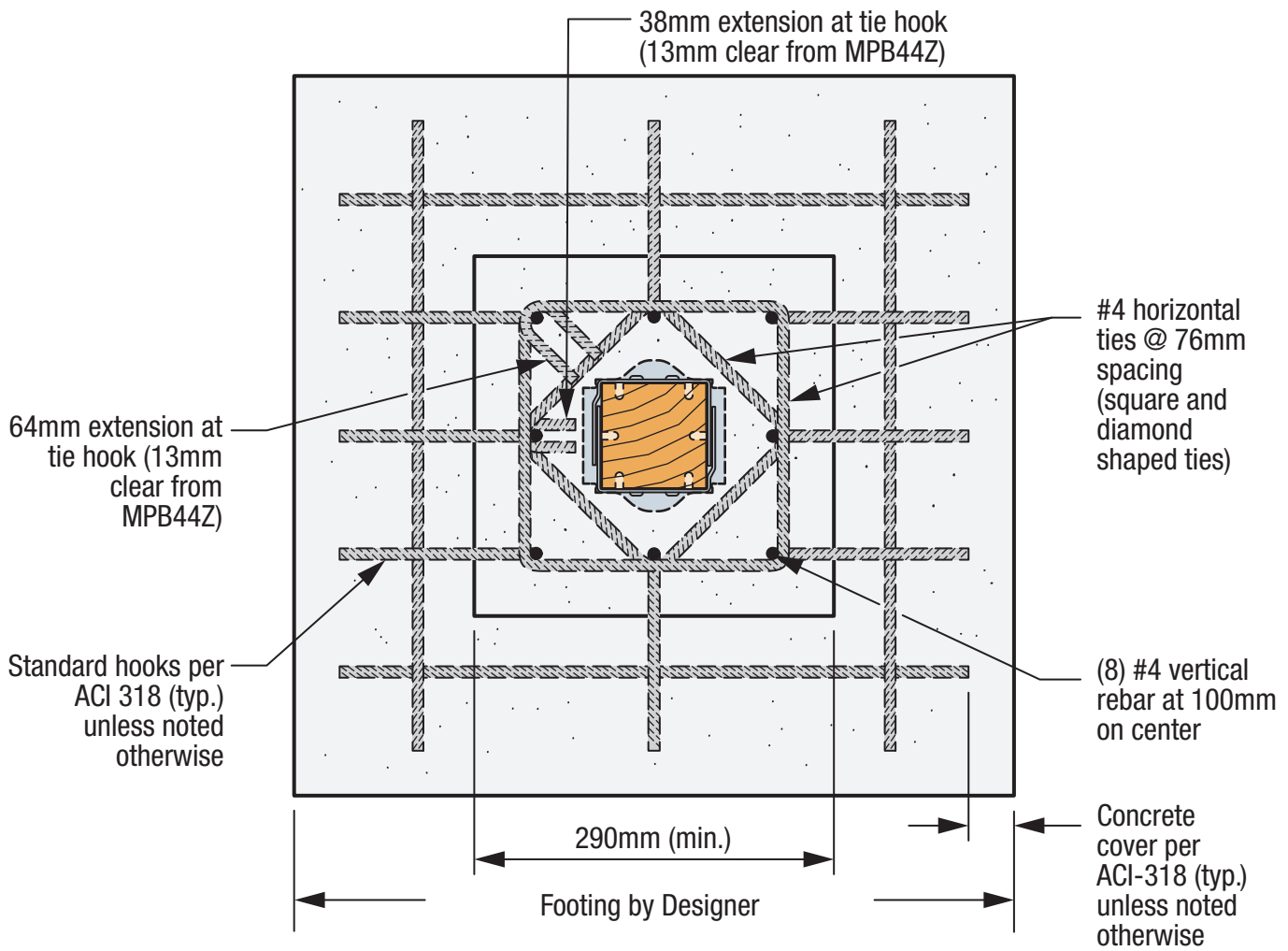
SIMPSON Strong-Tie® MPB44Z Reinforced Concrete Footing - Top View
