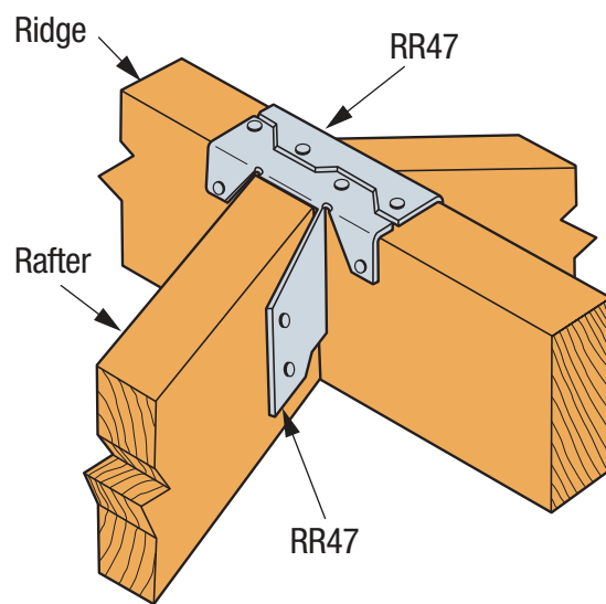
SIMPSON Strong-Tie® RR47 Ridge Rafter Connection
