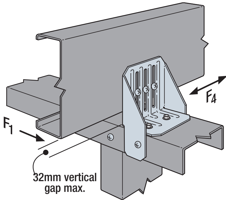
SIMPSON Strong-Tie® S/HTC4 Installation
