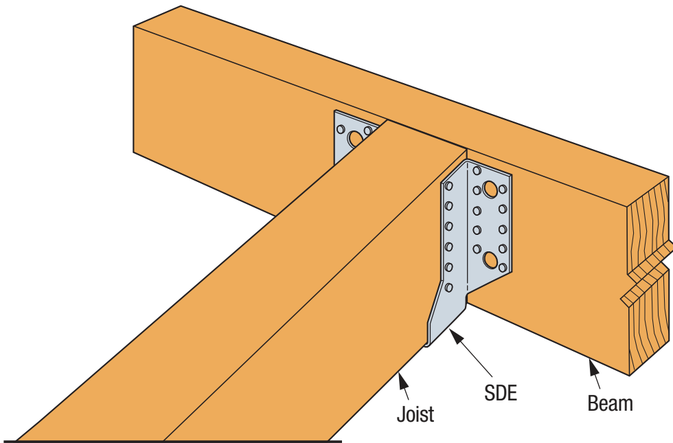
SIMPSON Strong-Tie® SDE Installation
