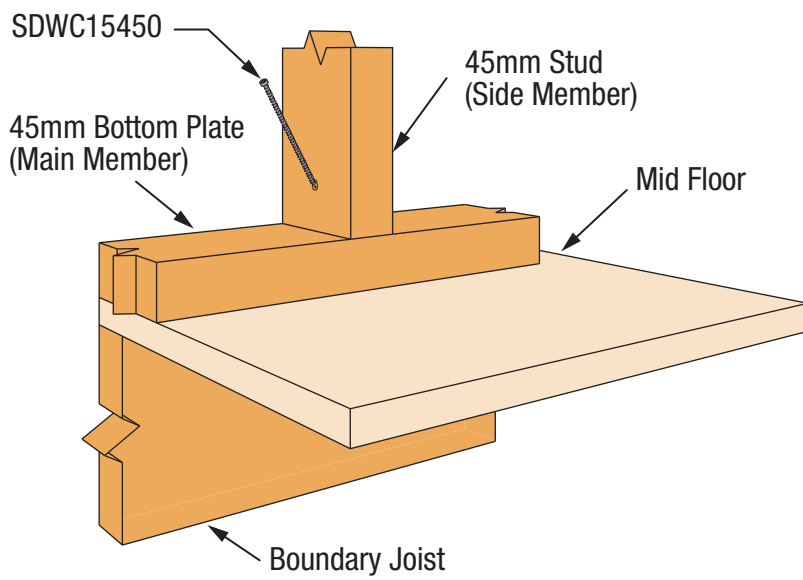
SIMPSON Strong-Tie® SDWC Stud-to-Bottom Plate Installation - Mid Floor
