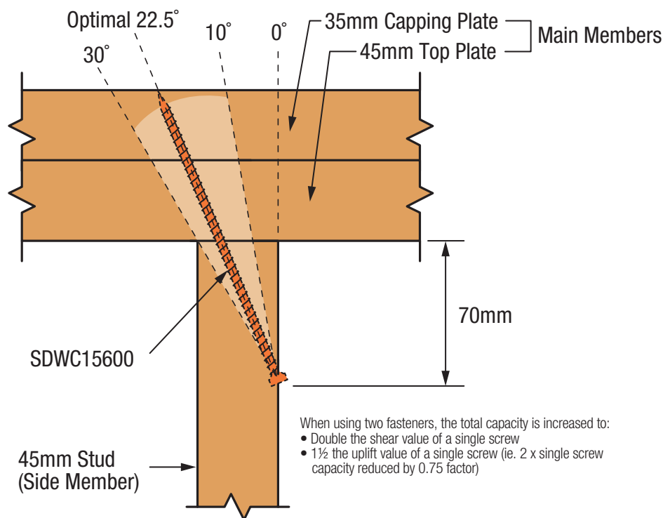
SIMPSON Strong-Tie® SDWC Stud-to-Top Plate Installation
