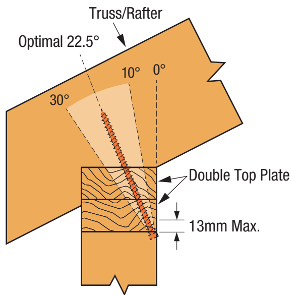
SIMPSON Strong-Tie® SDWC Truss/Rafter-to-Top Plate (double) Installation - Cross Section
