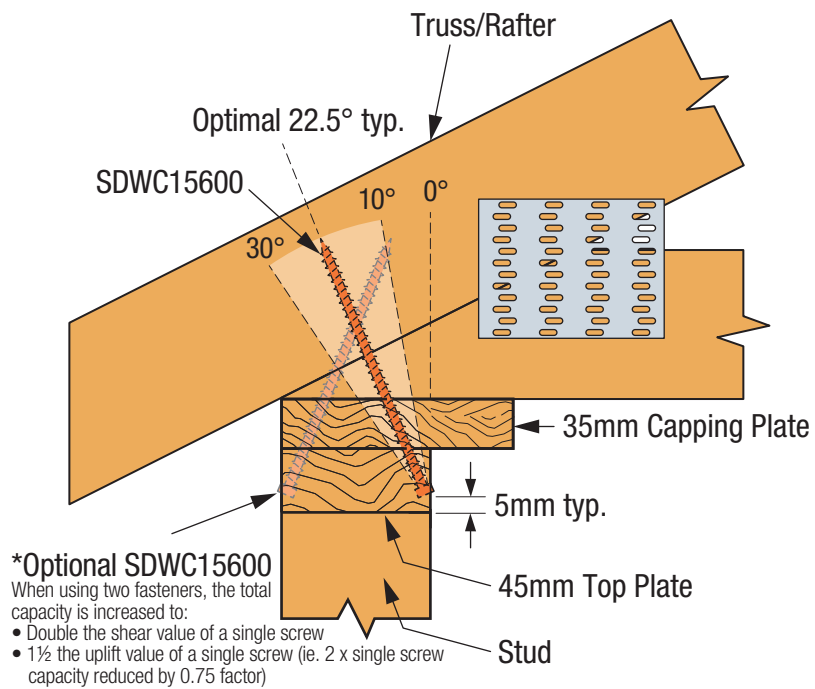
SIMPSON Strong-Tie® SDWC Truss/Rafter-to-Top Plate Installation - Cross Section
