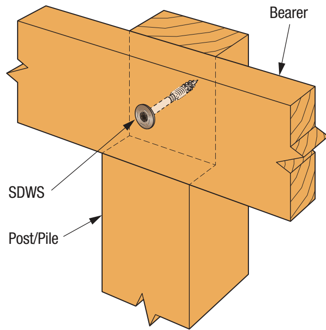
SIMPSON Strong-Tie® SDWS Bearer-to-Post/Pile Connection
