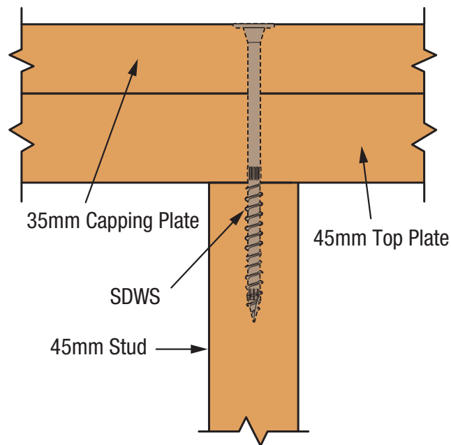
SIMPSON Strong-Tie® SDWS Stud-to-Top Plate - Cross Section
