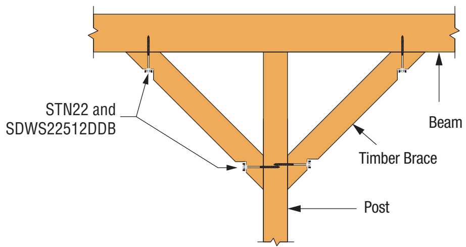
SIMPSON Strong-Tie® Timber Brace with STN22 + SDWS22512DDB
