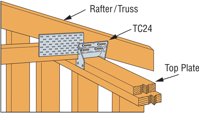
SIMPSON Strong-Tie® TC24 Installation
