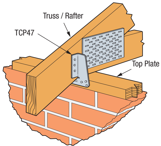
SIMPSON Strong-Tie® TCP Installation on Masonry Wall
