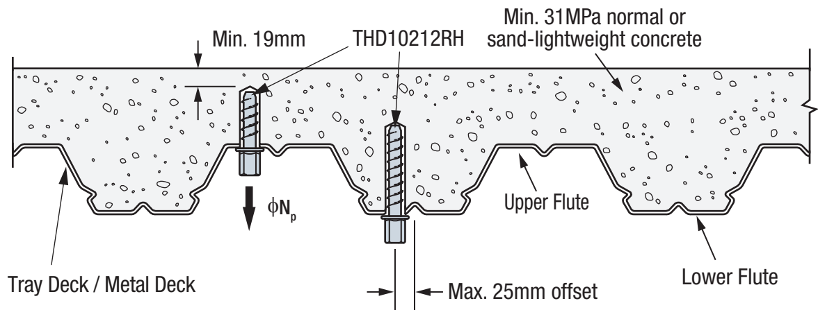
SIMPSON Strong-Tie® Titen HD Threaded Rod Hanger Fastening on Tray Deck / Metal Deck
