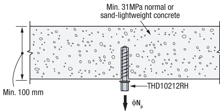
SIMPSON Strong-Tie® Titen HD Threaded Rod Hanger Installation in Concrete
