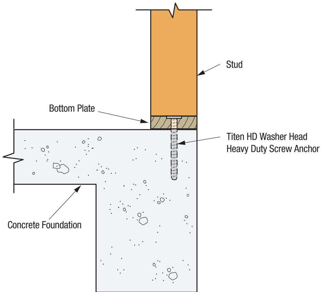
SIMPSON Strong-Tie® Titen HD Washer Head Bottom Plate Fixing - Cross Section
