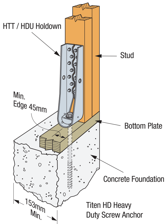
SIMPSON Strong-Tie® Titen HD With HTT/HDU Holddown Bottom Plate Fixing
