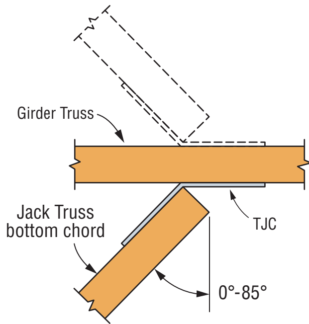
SIMPSON Strong-Tie® TJC Back-to-Back Installation
