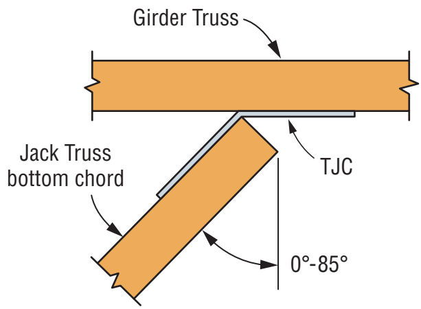
SIMPSON Strong-Tie® TJC Standard Installation - Top View
