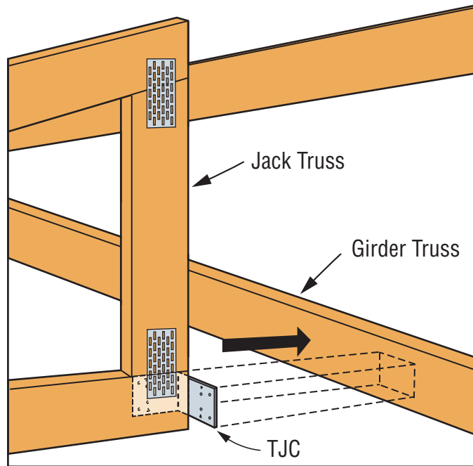
SIMPSON Strong-Tie® TJC Standard Installation
