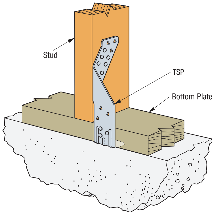
SIMPSON Strong-Tie® TSP Stud-to-Bottom Plate Tie Down
