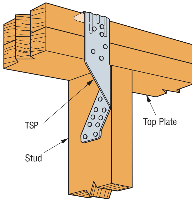
SIMPSON Strong-Tie® TSP Stud-to-Top Plate Tie Down
