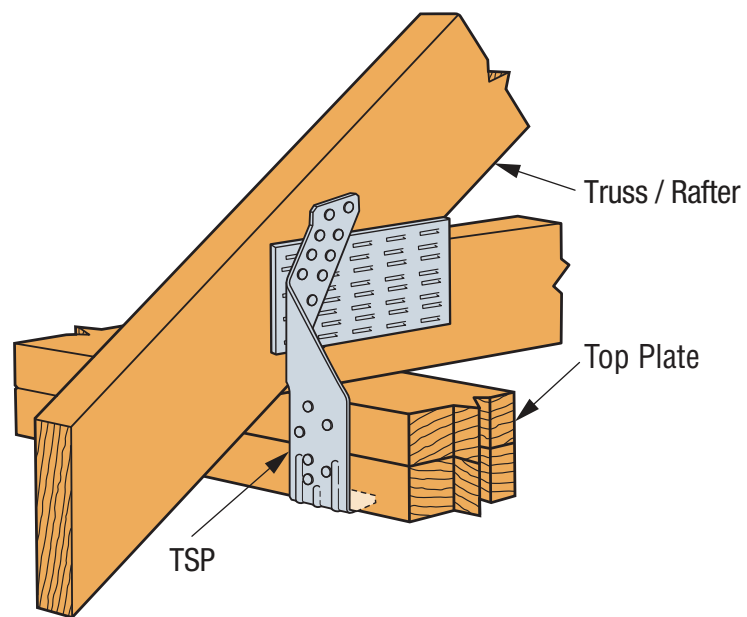
SIMPSON Strong-Tie® TSP Truss/Rafter-to-Top Plate Tie Down
