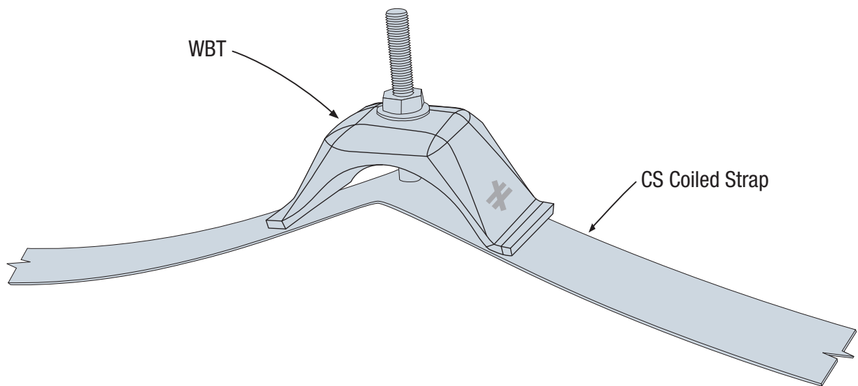
SIMPSON Strong-Tie® WBT Installation with CS Coiled Strap
